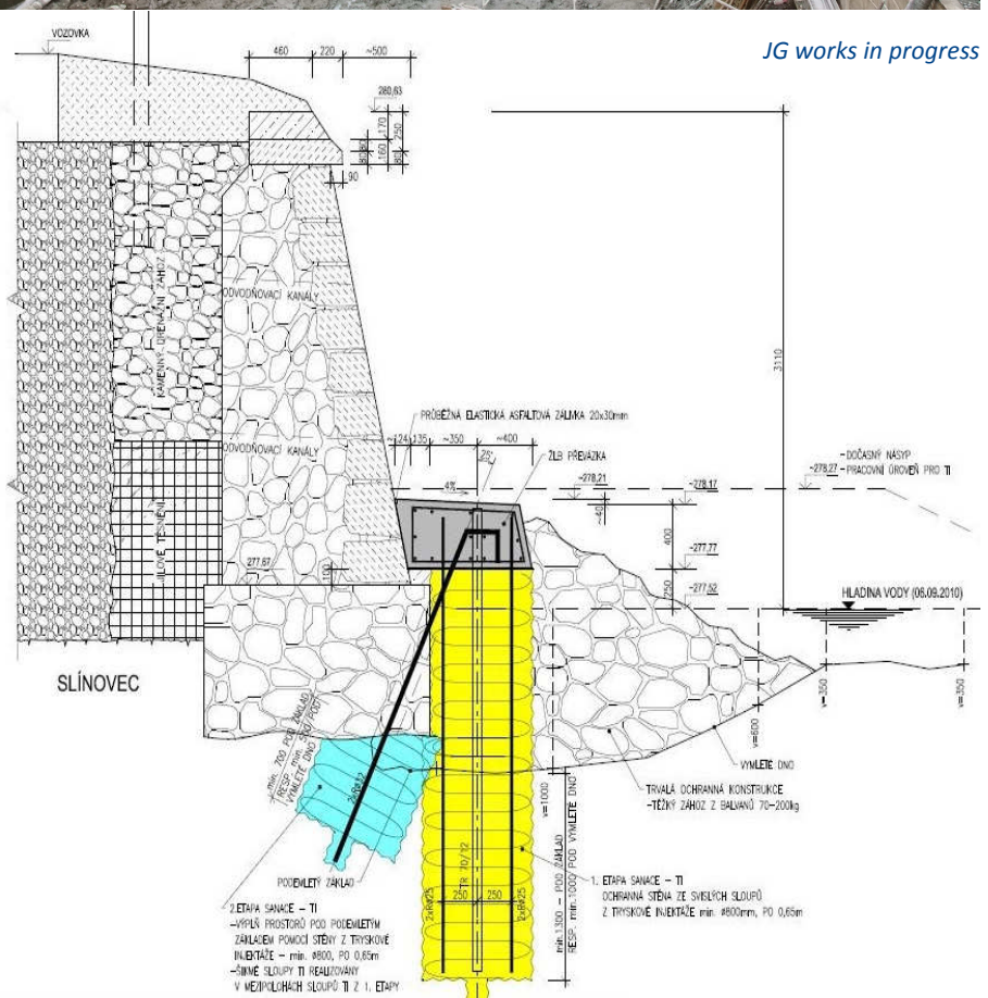
Layout of reconstruction supporting wall
