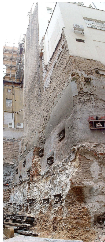
Underpinning of adjacent buildings
