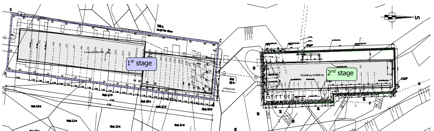
Layout of cut-off walls
